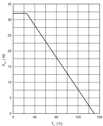
Fig. 1 Power dissipation
